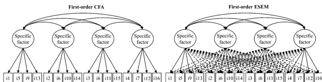
Figure 1. Schematic comparison of multi-factor correlated CFA and ESEM models. Note. CFA = confirmatory factor analysis; ESEM = exploratory structural equation modelling. Circles represent latent variables, and squares represent scale items. One-headed full arrows represent factor loadings, one-headed dashed arrows represent cross-loadings, and two-headed arrows represent factor correlations
